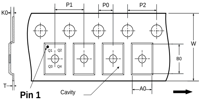
TAPE DIMENSIONS
